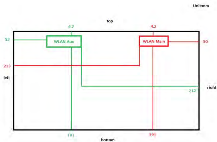
Fig.10 Antenna location of EUT
