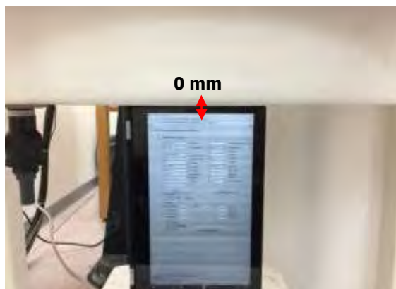
Fig.6 EUT Left side to flat phantom (tablet mode)
