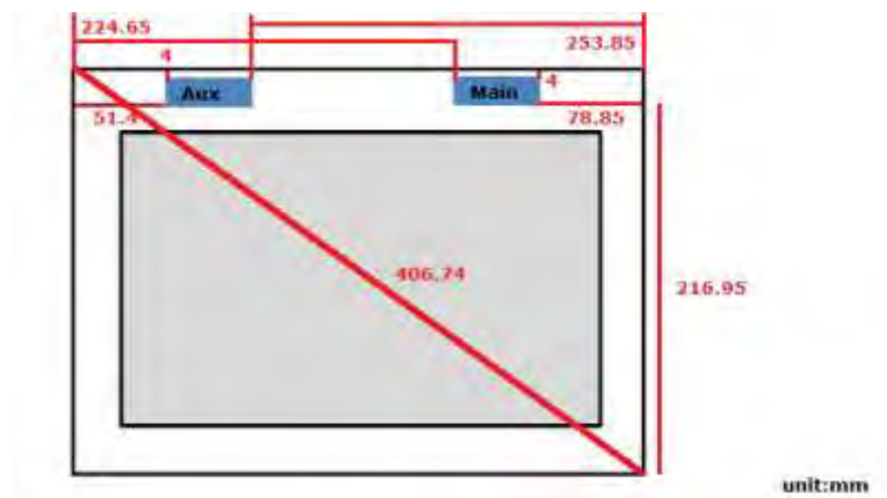
Fig.12 Antenna location (front view of tablet mode)
