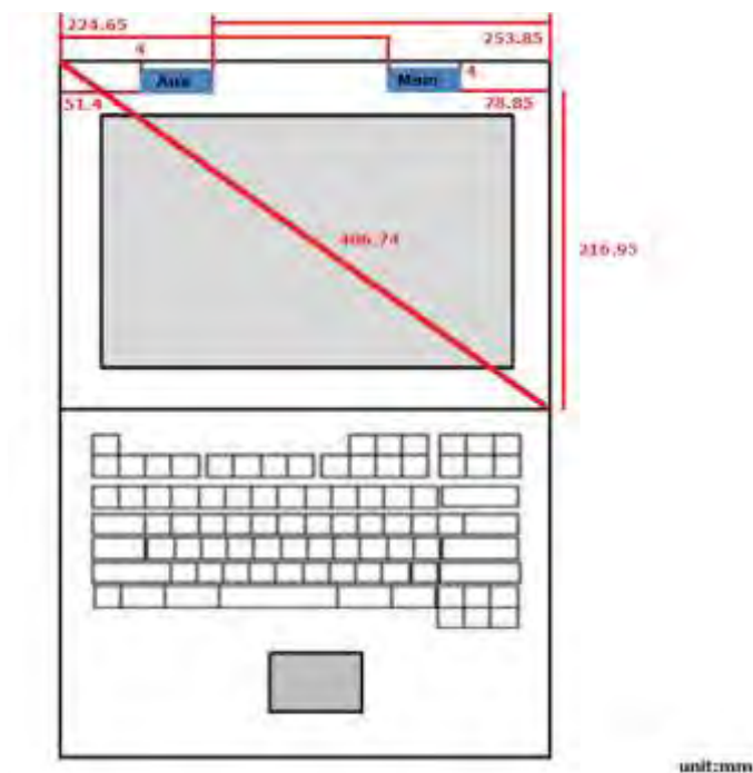
Fig.11 Antenna location (front view of laptop mode)
