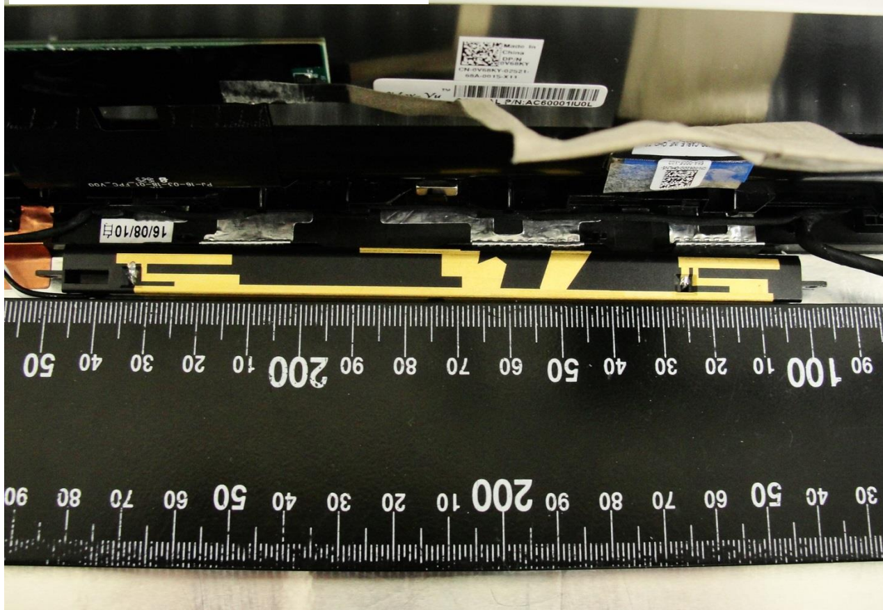
WLAN Main and Aux. Antenna for Sample 1
