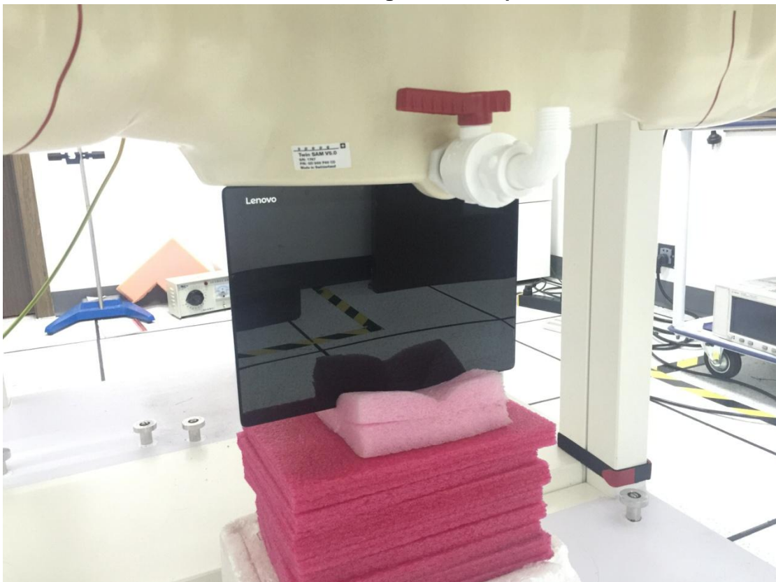
2.4 Tablet Mode-Edge_1 with Gap 0mm
