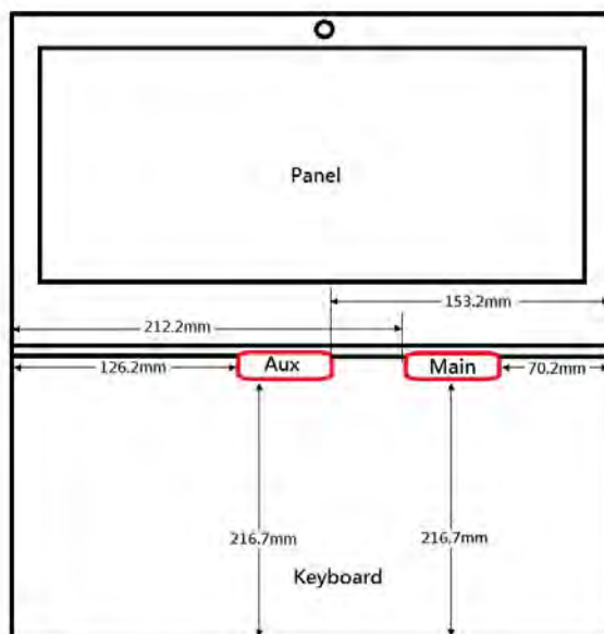
Fig.7 Antenna position of EUT (Front view)
