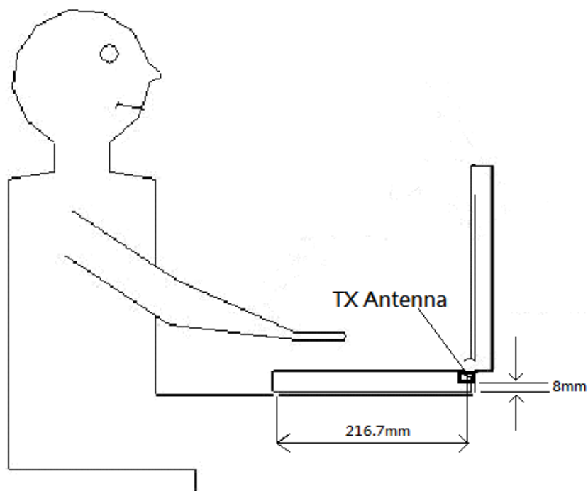
Fig.8 Antenna-to-user separation distance
