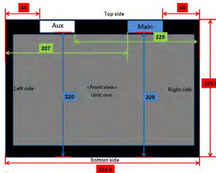
Fig.8 Antenna location of tablet mode
