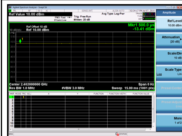
3DH5 2402MHz
