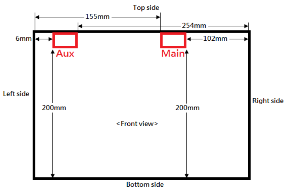
Front view of tablet
