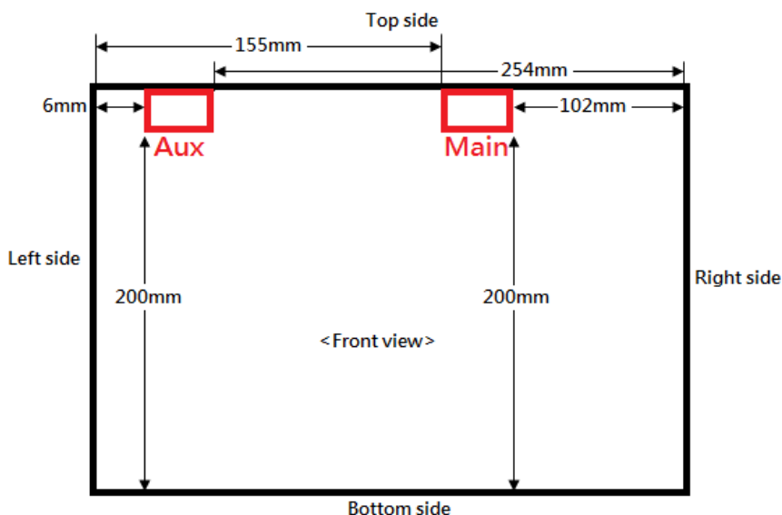
Fig.8 Antenna position of EUT (Front view)
