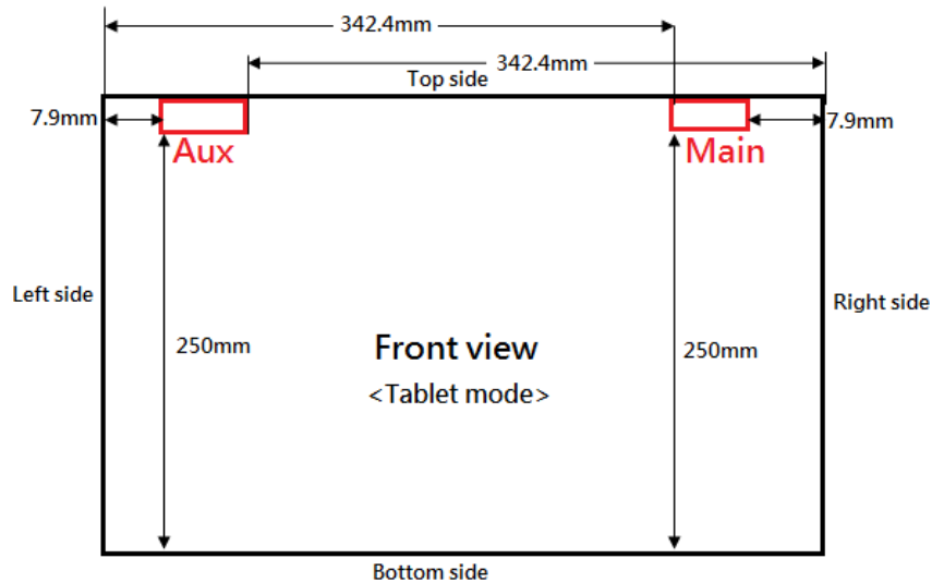
Fig.9 Antenna position of EUT (Back view)
