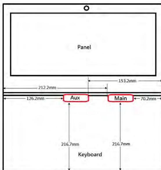
Fig.6 Laptop mode view of EUT
