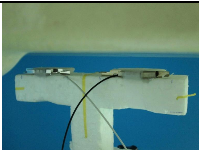
Rear Face of EUT with 1 cm Gap
