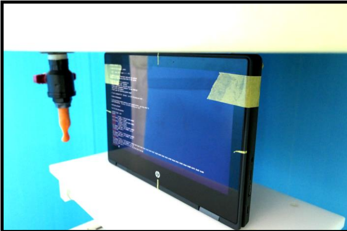
Body - Top Side of EUT at 0 mm
