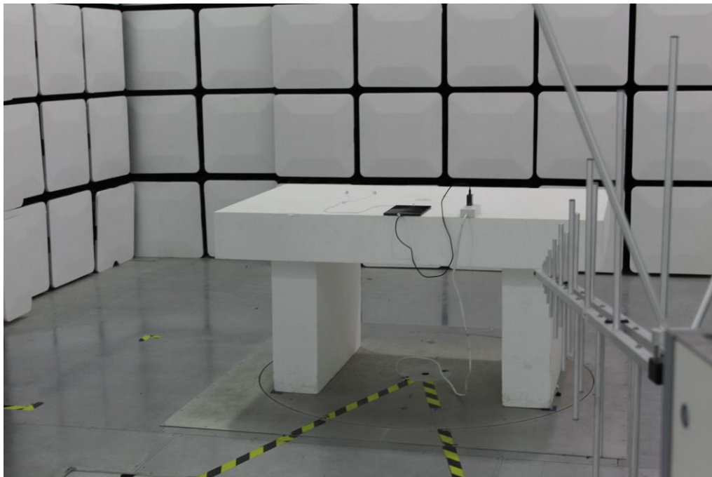
Setup for Unwanted Emissions that fall Outside of the Restricted Bands(Radiated) and Unwanted Emissions in the Restricted Bands (Radiated) above 1GHz
