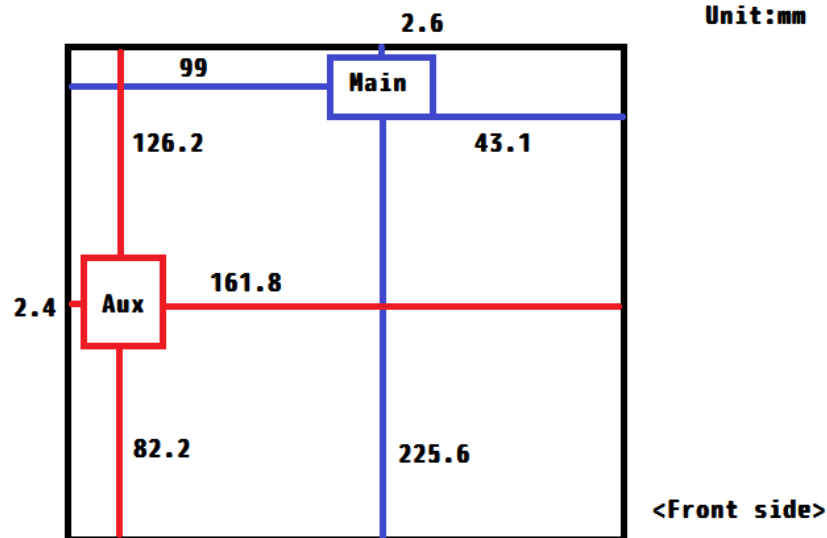
Fig.9 Antenna position of EUT
