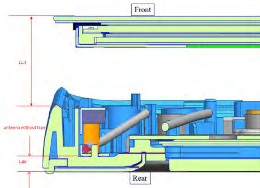
<The Distance information of Antenna to Front and Rear of Tablet PC>
