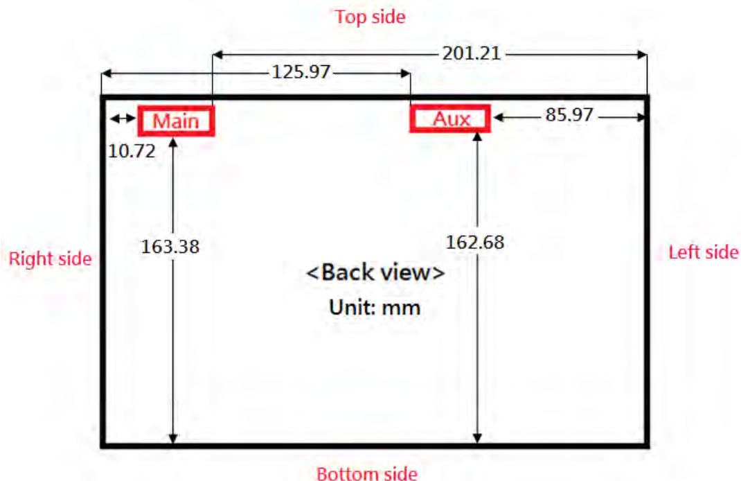
Fig.8 Antenna position of EUT (Front view)
