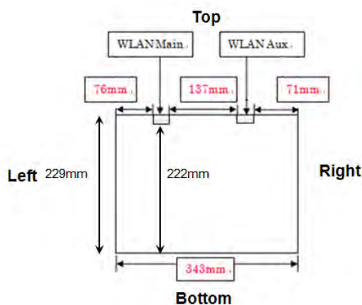
Fig.10 Antenna position (Front view of Tablet mode )
