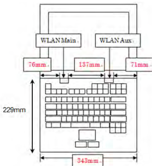
Fig.9 Antenna position ( Front view of Laptop mode)
