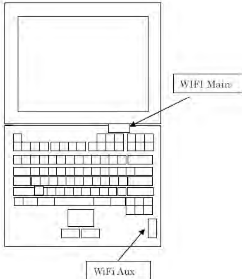
Fig.8 Antenna position of EUT (Front view)
