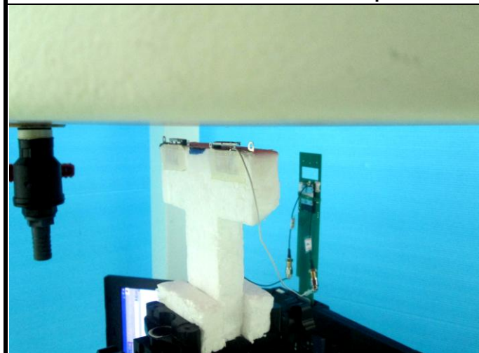
Top Side of EUT with 8 mm Gap
