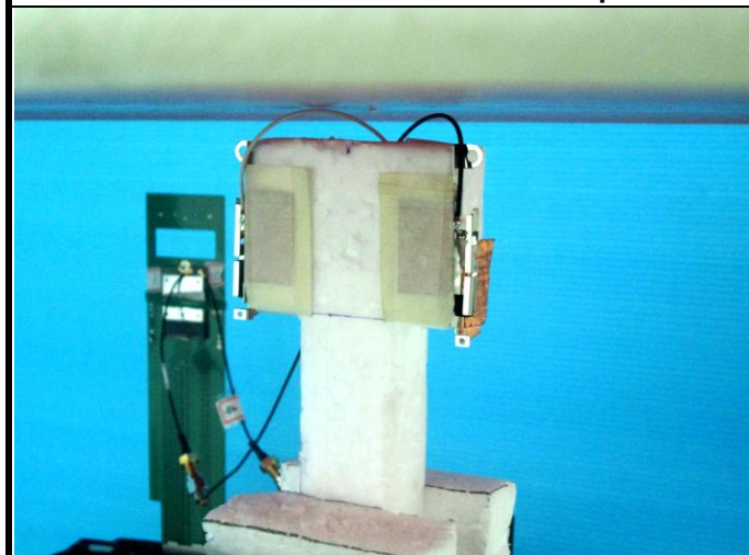
Left Side of EUT with 8 mm Gap
