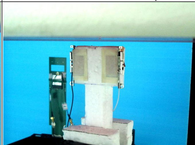
Right Side of EUT with 8 mm Gap
