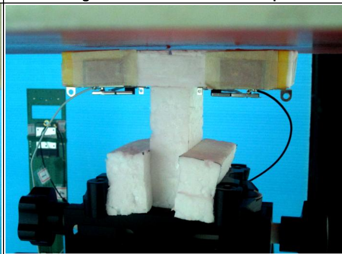
Bottom Side of EUT with 8 mm Gap
