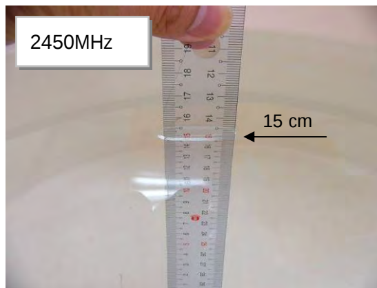
Fig.2.1 Flat (Body)
