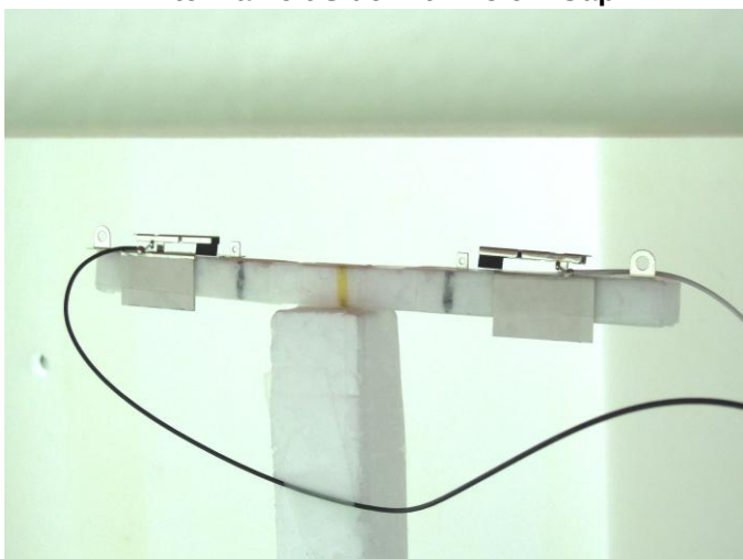
Antenna Top Side with 2.5 cm Gap
