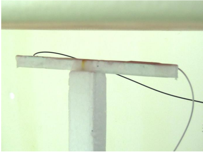
Antenna Front Face with 2.5 cm Gap
