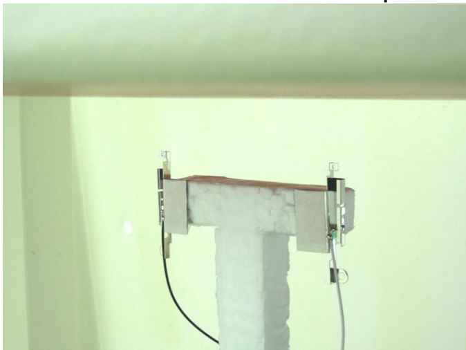
Antenna Left Side with 2.5 cm Gap
