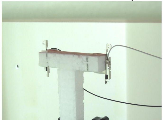
Antenna Right Side with 2.5 cm Gap
