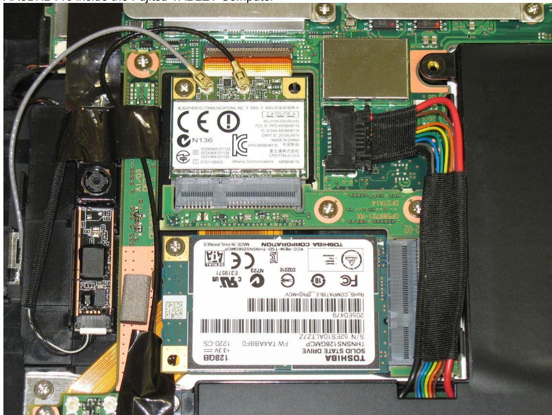
AR5BHB116 inside the Fujitsu TABLET Computer
