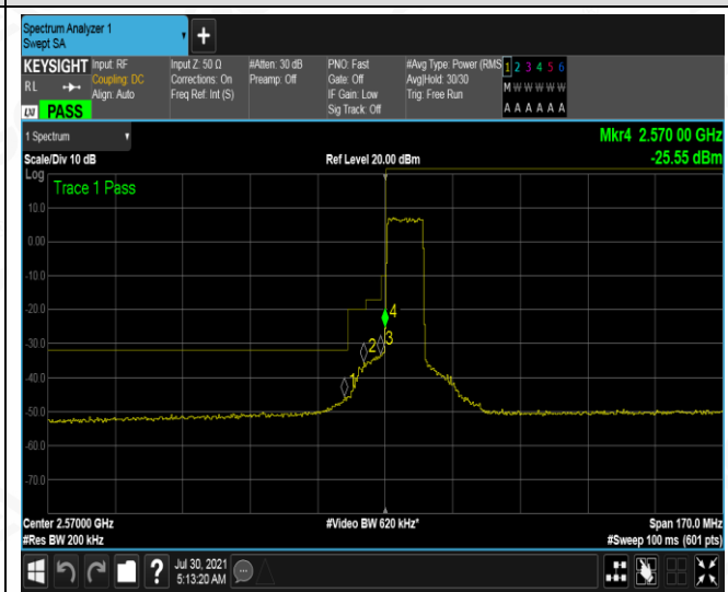
LCH_16QAM_50RB#0
