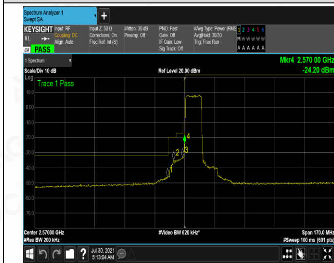
LCH_QPSK_50RB#0
