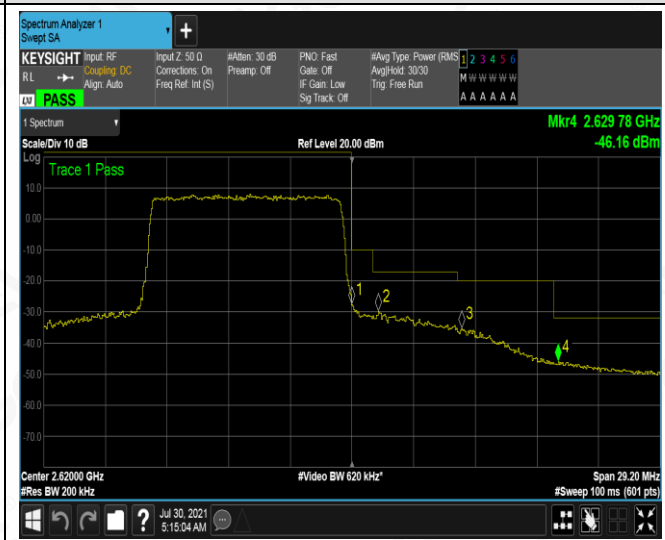
HCH_16QAM_50RB#0
