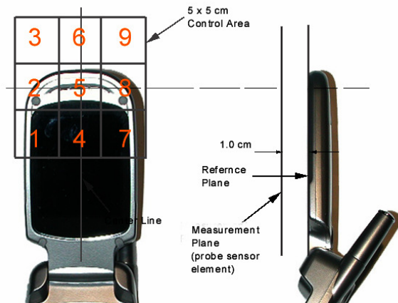
Figure 12 E/H-Field Emissions Test Setup Diagram
