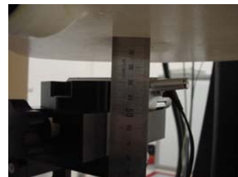
Fig. 20. Body SAR Test Setup with Holster
