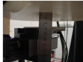
Fig. 21. Body SAR Test Setup with Holster
