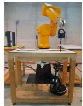
Figure 1. SAR System
