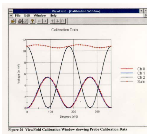
Figure 26 ViewField Calibration Window showing Probe Calibration Data
