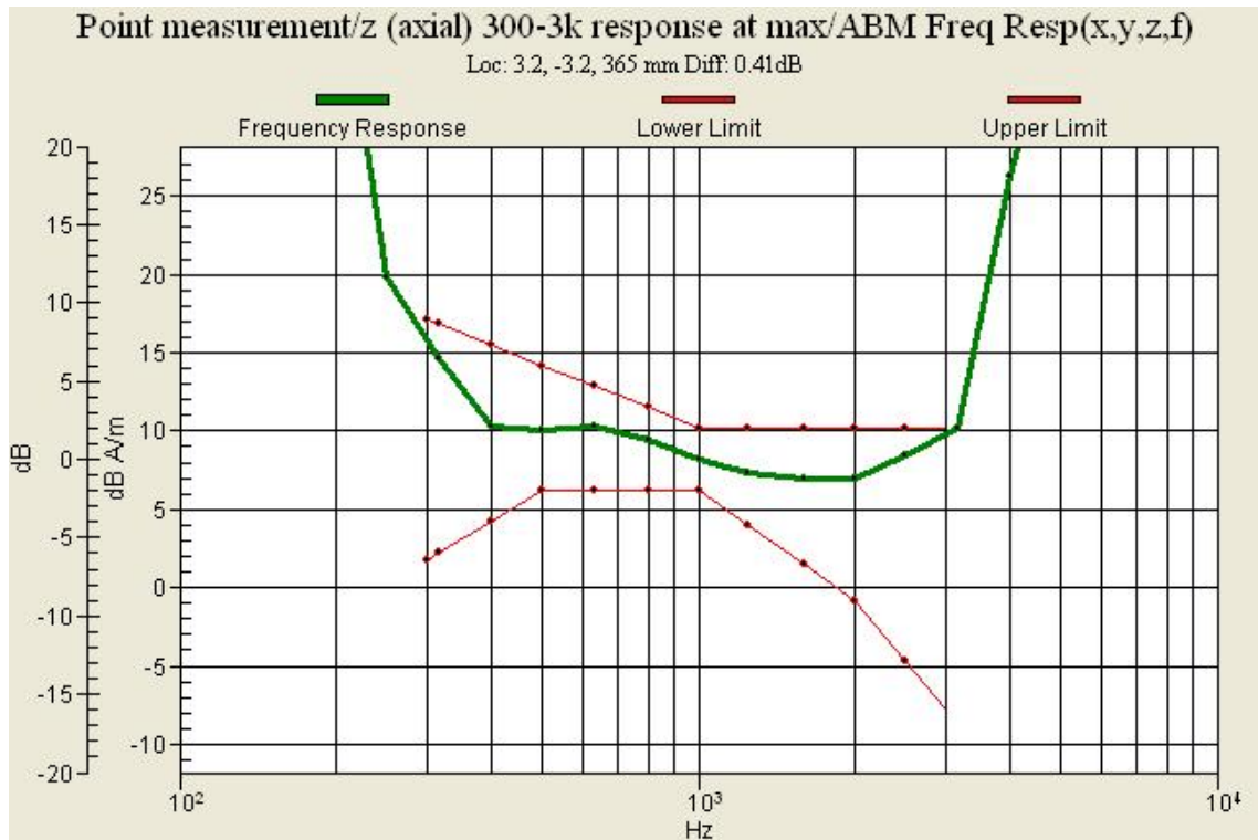
Graph 4 : PCS 1900 (CH 25) Frequency Response
