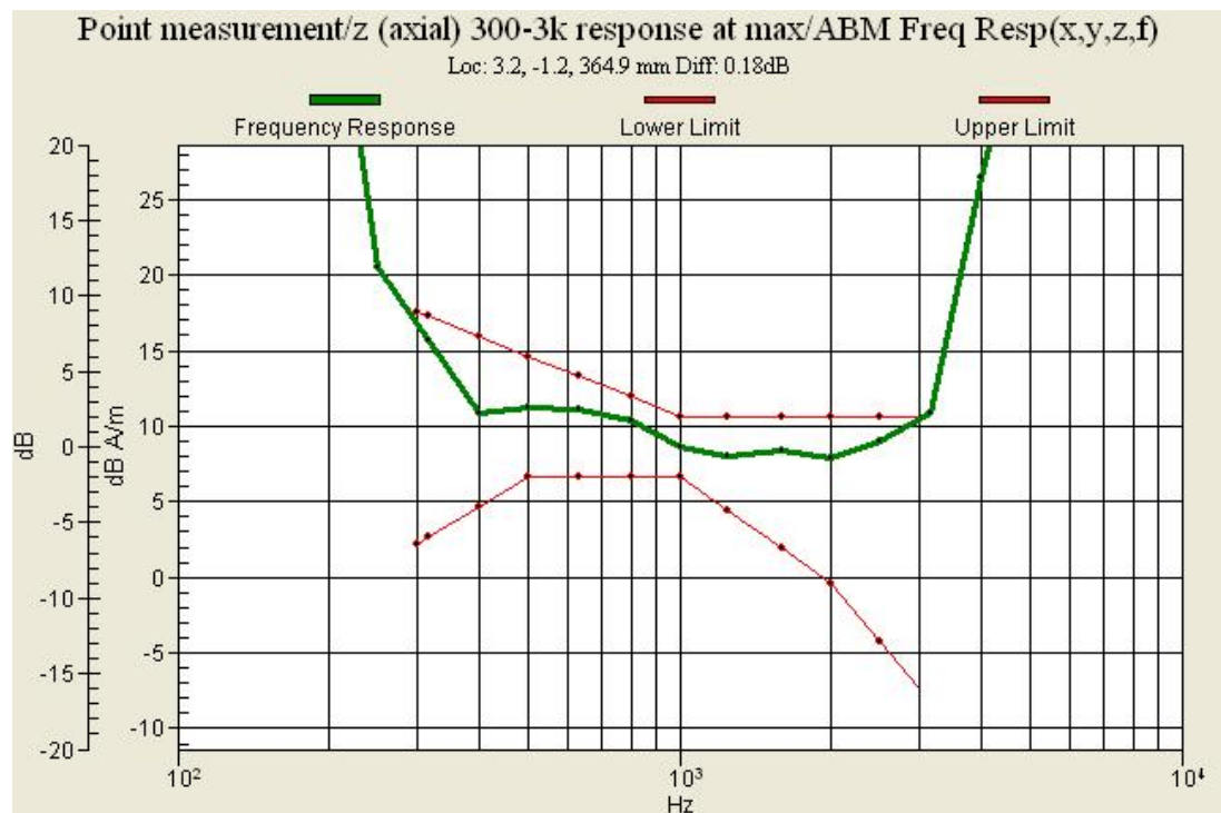
Graph 2 : CDMA 800 (CH 384) Frequency Response
