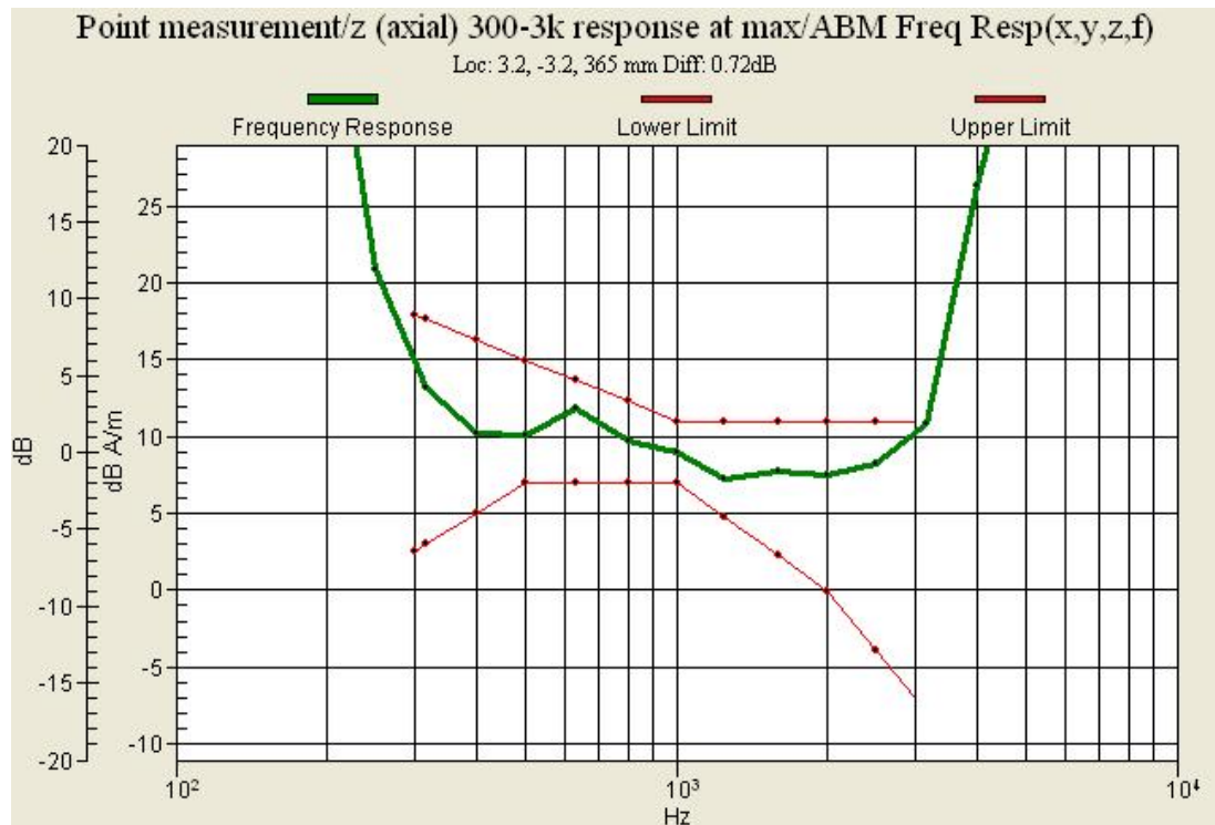
Graph 1 : CDMA 800 (CH 1013) Frequency Response
