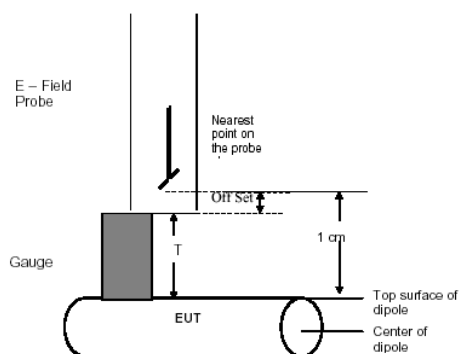
Figure 4. Gauge Block with E-Field Probe
