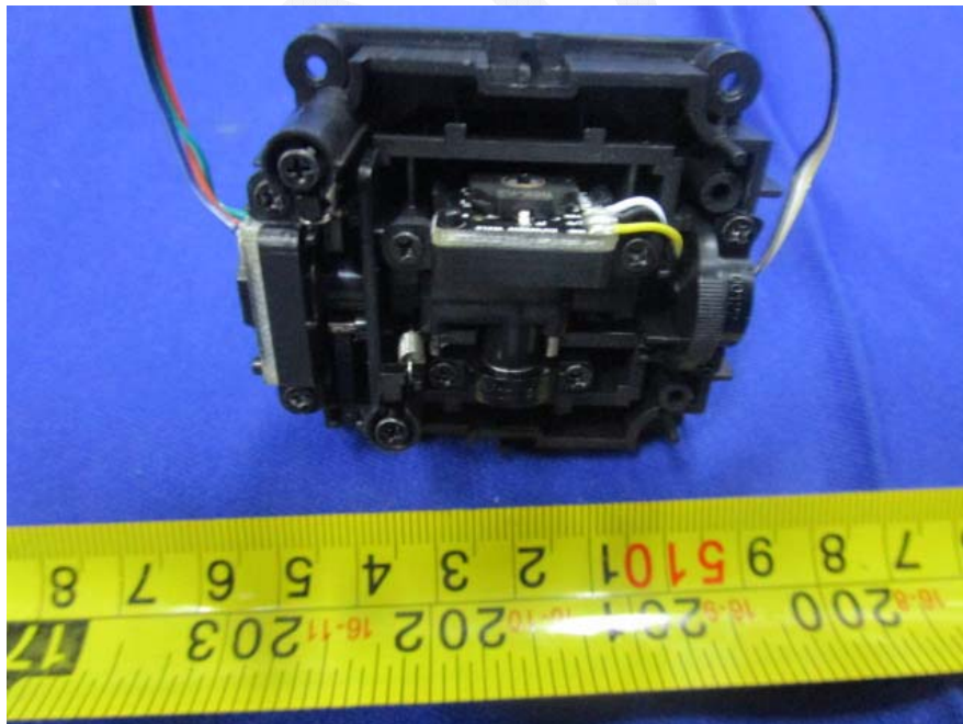
EUT – Rock Bar Bottom View
