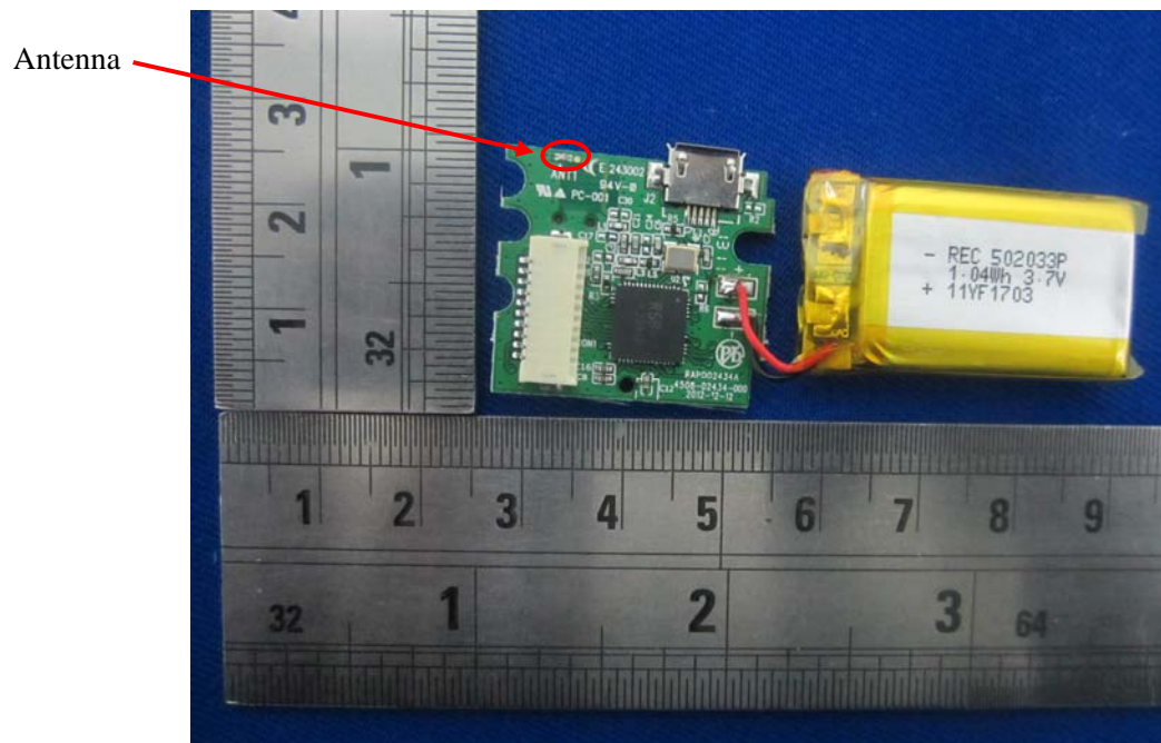
EUT –Main Board With Battery Bottom View
