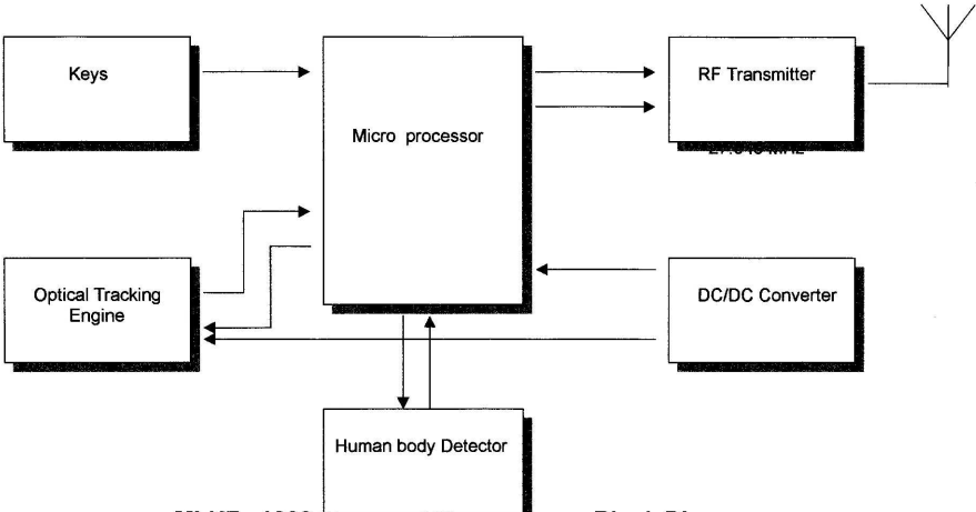
MLKF 1000 Cordless Optical mouse Block Diagram
