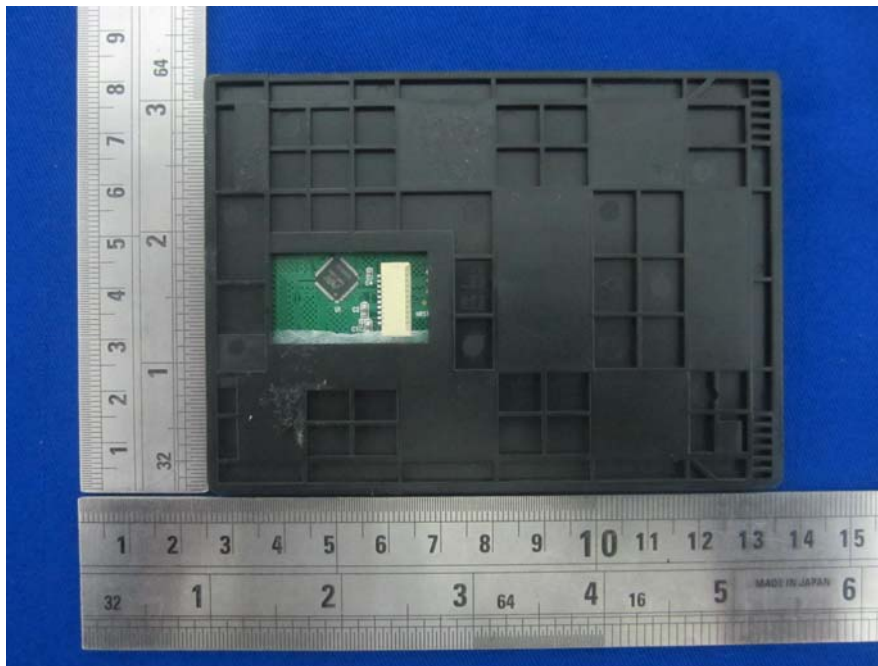
EUT –Touch Box Bottom View
