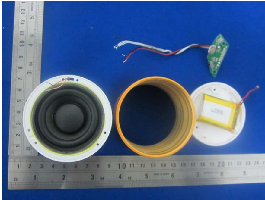
EUT – Speaker Off View
