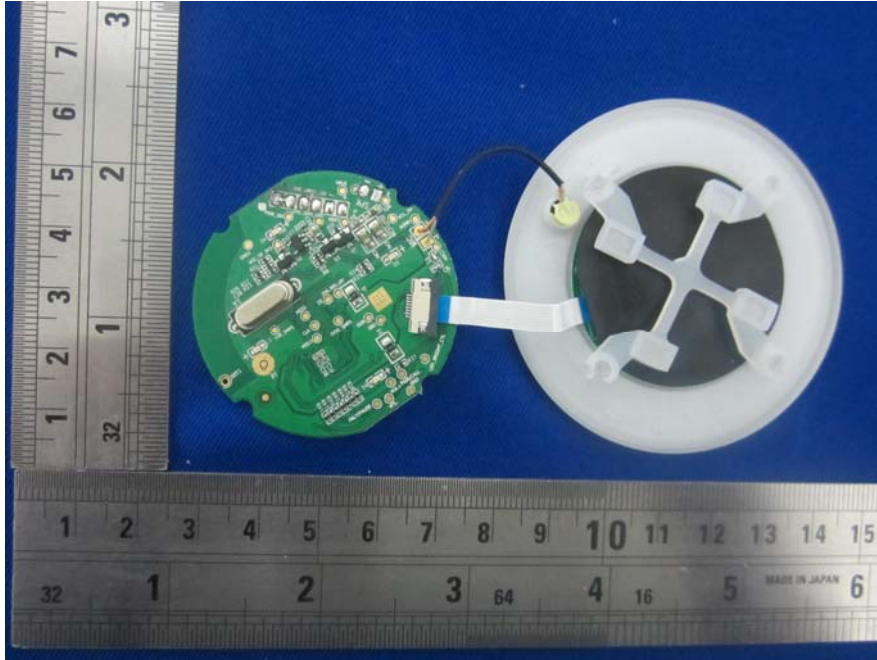
EUT – Top Cover View
