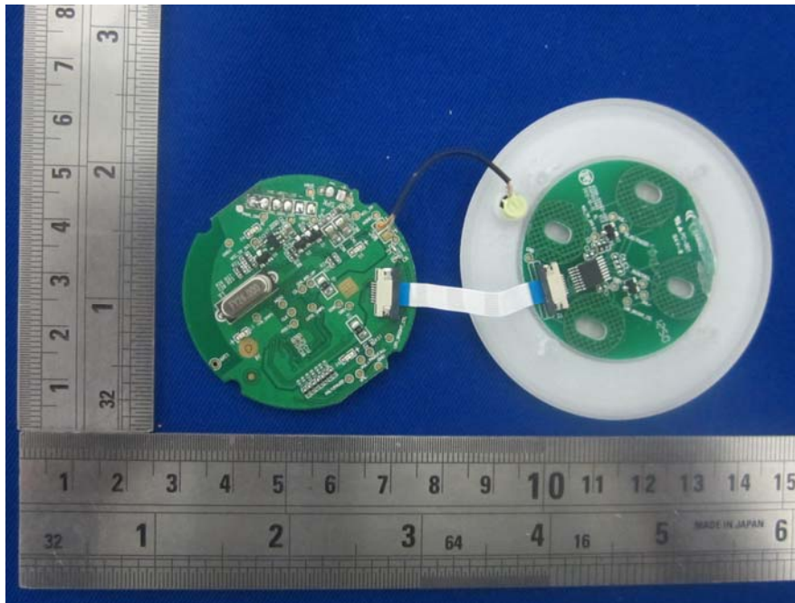
EUT – Top Cover Board View
