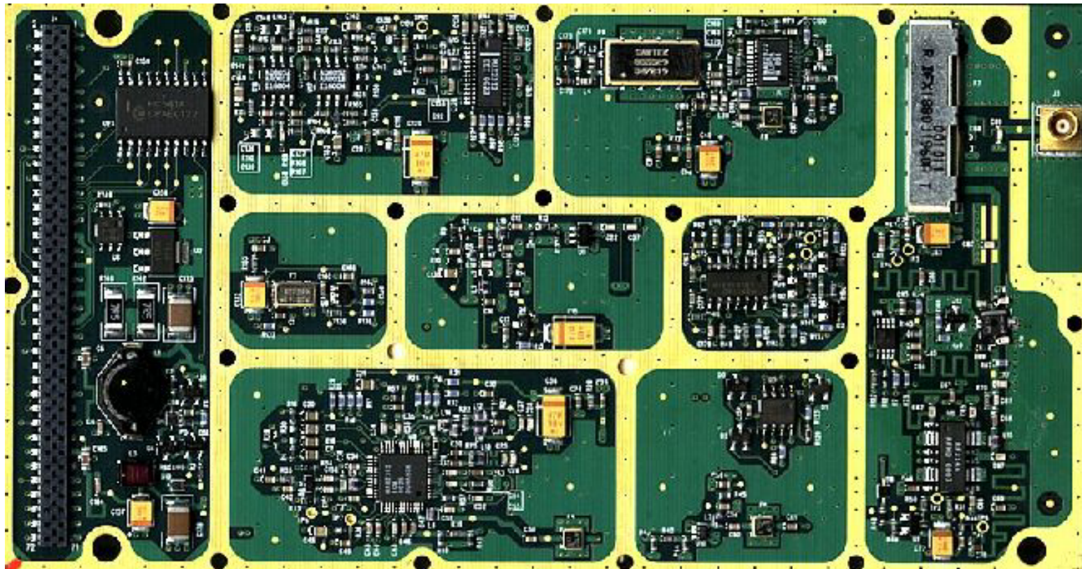
RF Module Board Top Side with no shield
