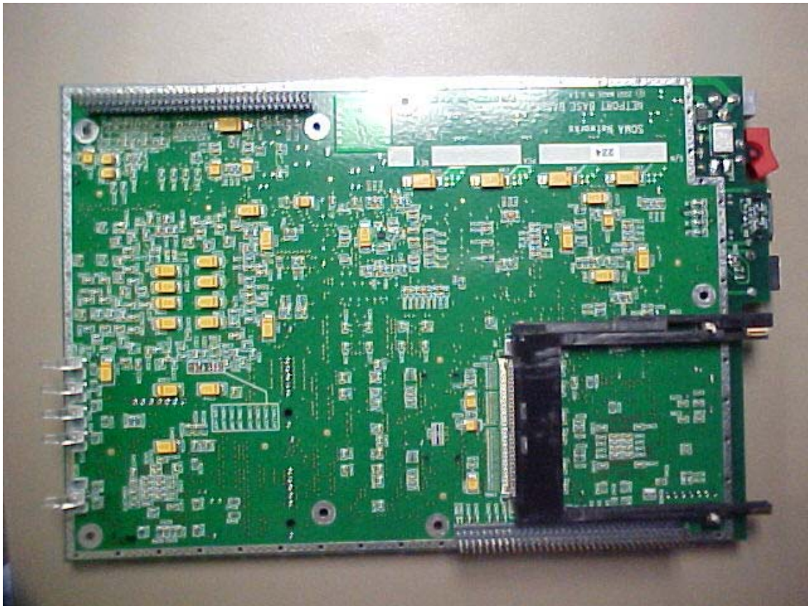
SOLDER SIDE OF BASEBAND CARD
