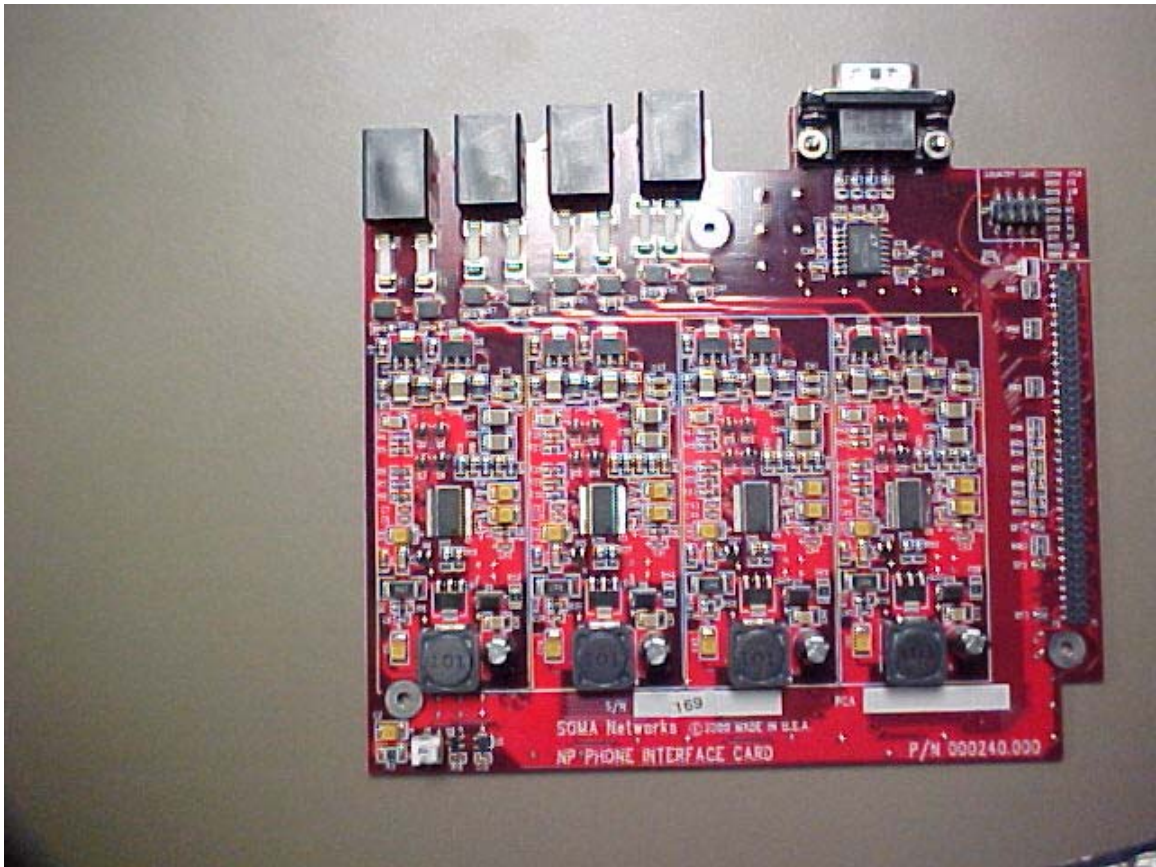
COMPONENT SIDE OF PHONE INTERFACE CARD
