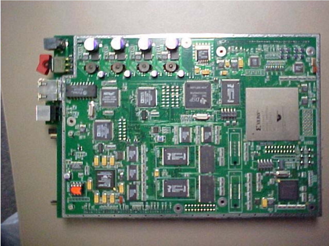
BASEBAND CARD COMPONENT SIDE VIEW
