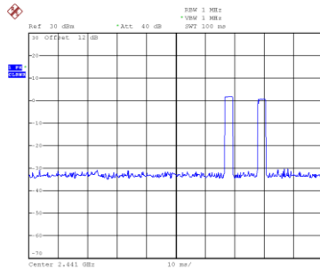
CH39-2DH5
