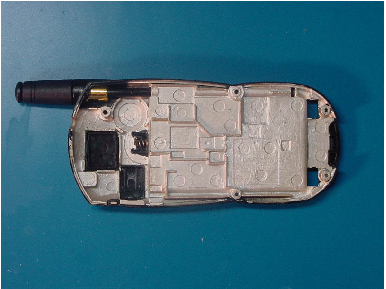
PHOTOGRAPH 6: REAR INSIDE
