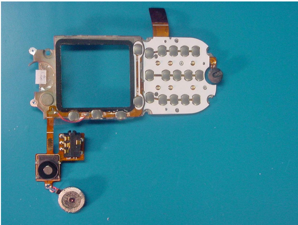
PHOTOGRAPH 7: KEYBOARD FRONT
