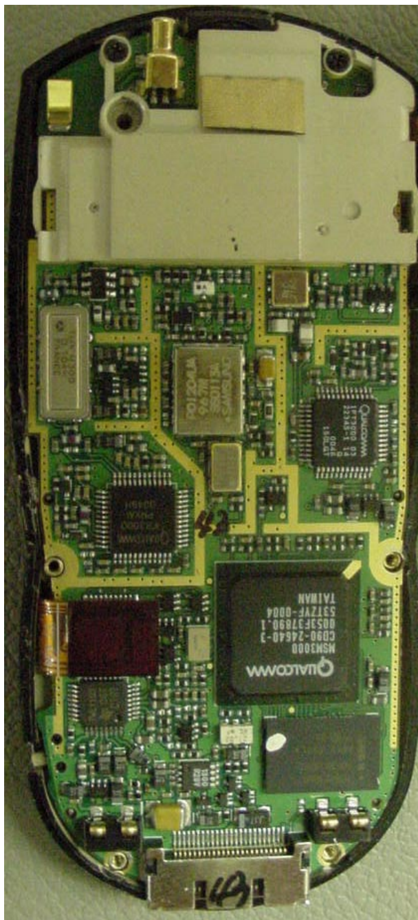
PHOTOGRAPH 14: INSIDE REAR SHOWING PCB WITH GASKET
