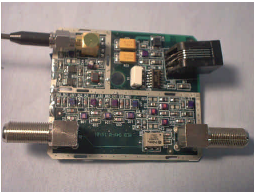
Ucentric Home Server (splitter – top without cans) FCC ID: POPFMTRANSMITTER
