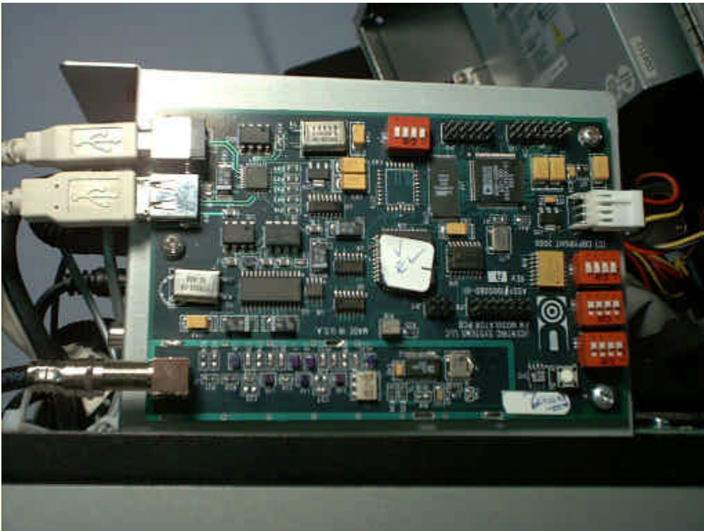
Ucentric Home Server (base unit transmitter board - top) FCC ID: POPFMTRANSMITTER
