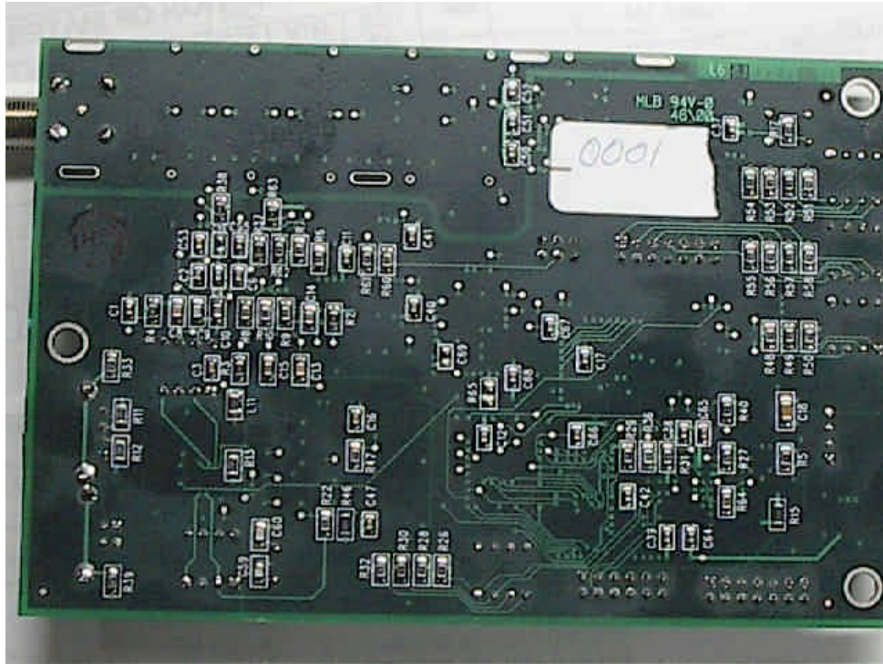
Ucentric Home Server (base unit transmitter board - bottom) FCC ID: POPFMTRANSMITTER
