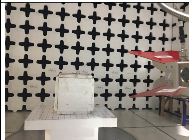
Radiated Emissions Front (Above 1 GHz)
