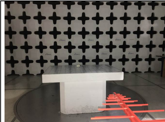
Radiated Emissions Front (Below 1 GHz)
