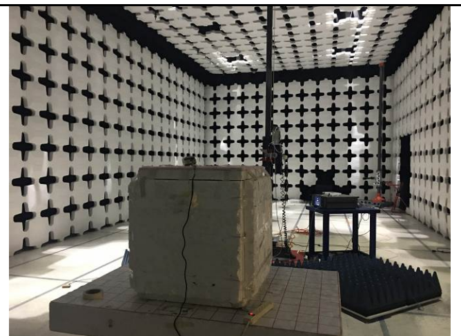
Radiated Emissions Rear (Above 1 GHz)
