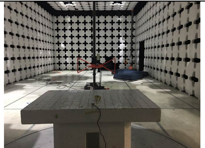
Radiated Emissions Rear (Below 1 GHz)
