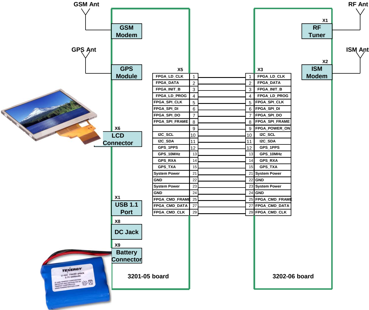
Block diagram of QS Navigator
