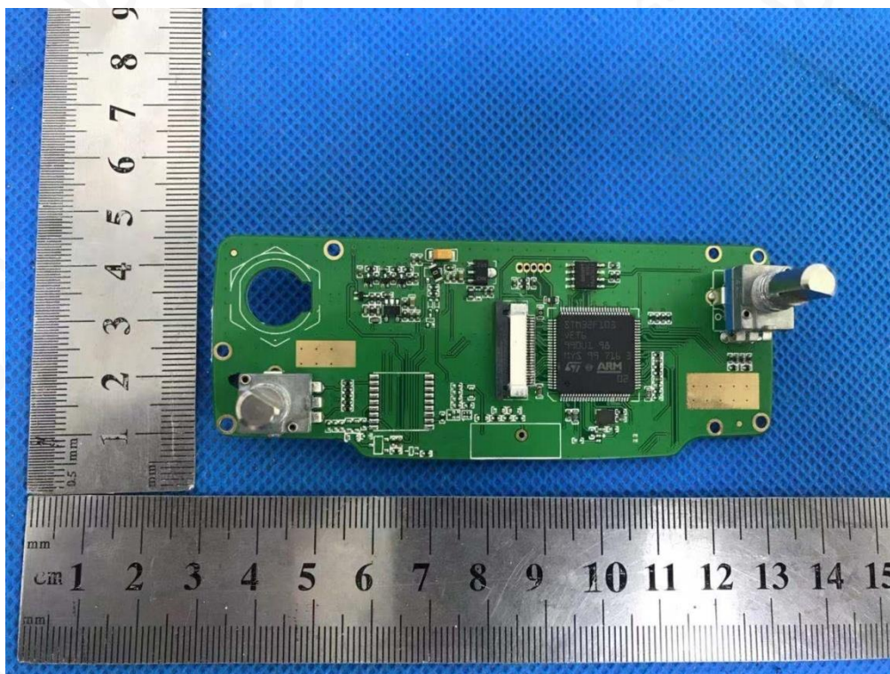
INTERNAL VIEW-3 OF EUT-2
