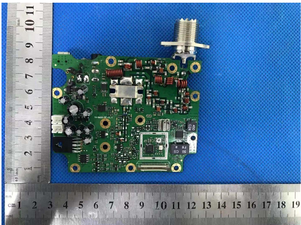
INTERNAL VIEW-2 OF EUT-1
