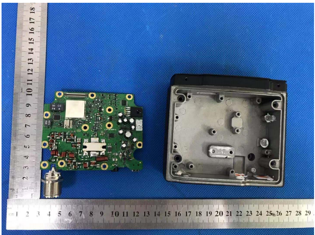
OPEN VIEW-3 OF EUT-1
