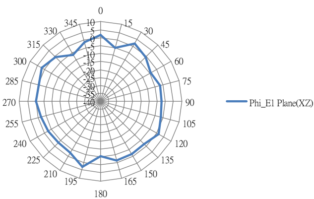
Phi_E1 Plane(XZ)
