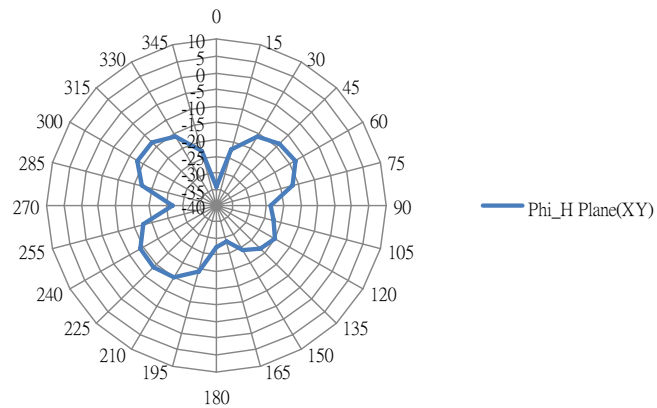
Phi_H Plane(XY)
