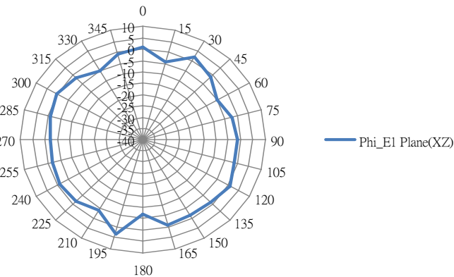
Phi_E1 Plane(XZ)
