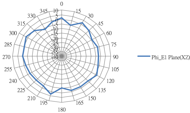
Phi_E1 Plane(XZ)
