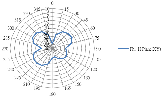
Phi_H Plane(XY)
