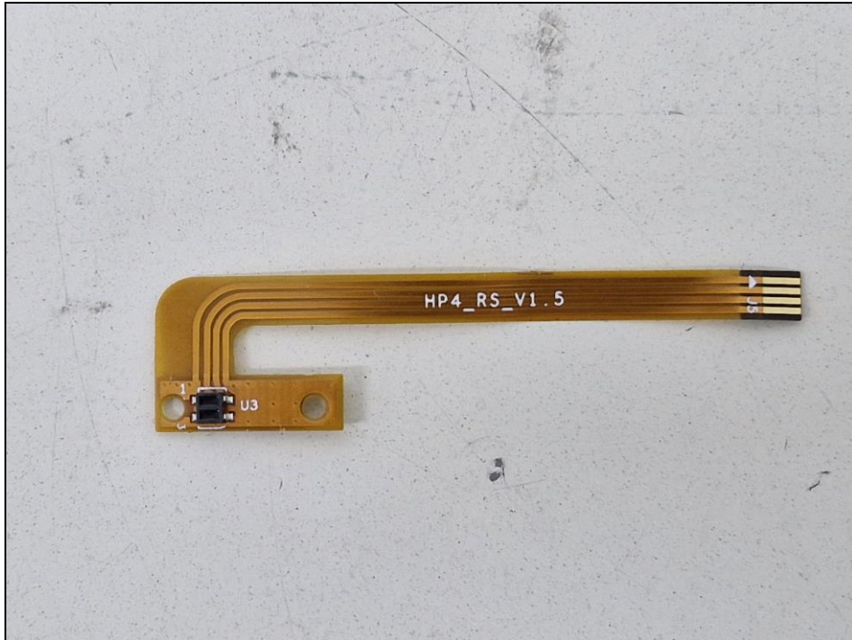
Top view of Sub2 PCB
