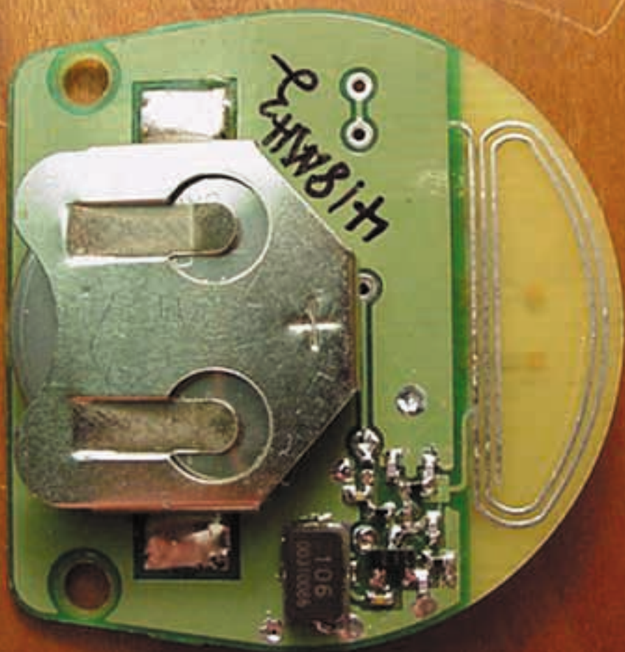
418MHz circuit back
