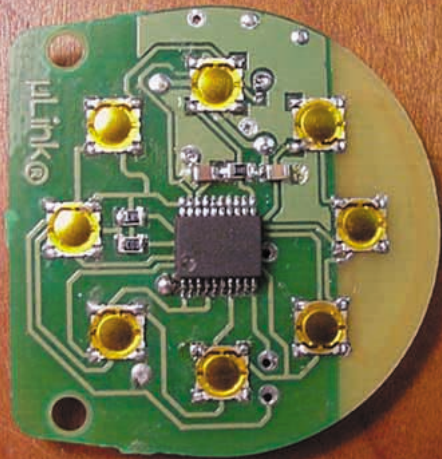
433MHz circuit top
