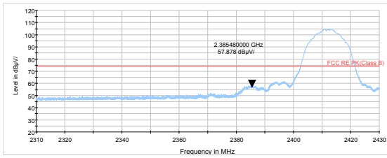
802.11b-Channel 1 Peak
