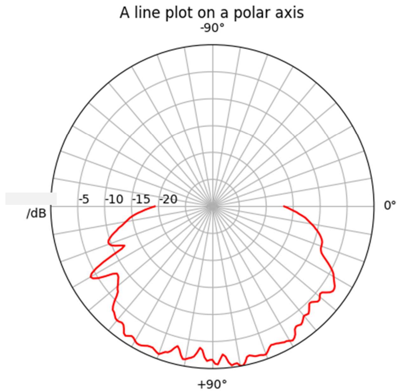
Horizontal polar plot of Tx antenna
