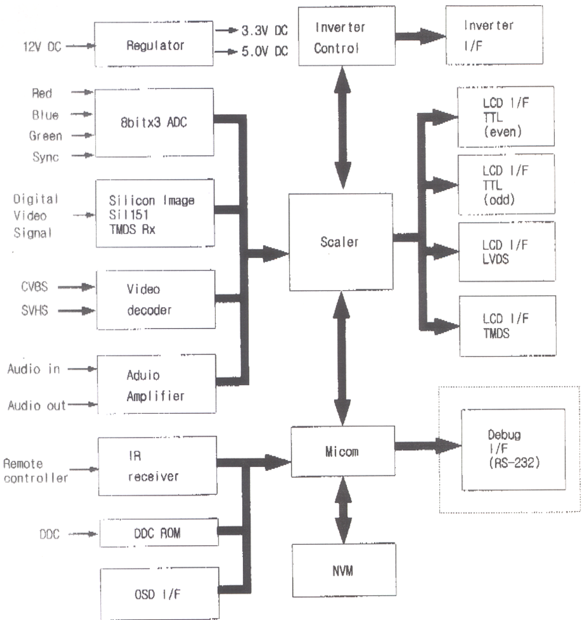
3-3 Block Diagram
